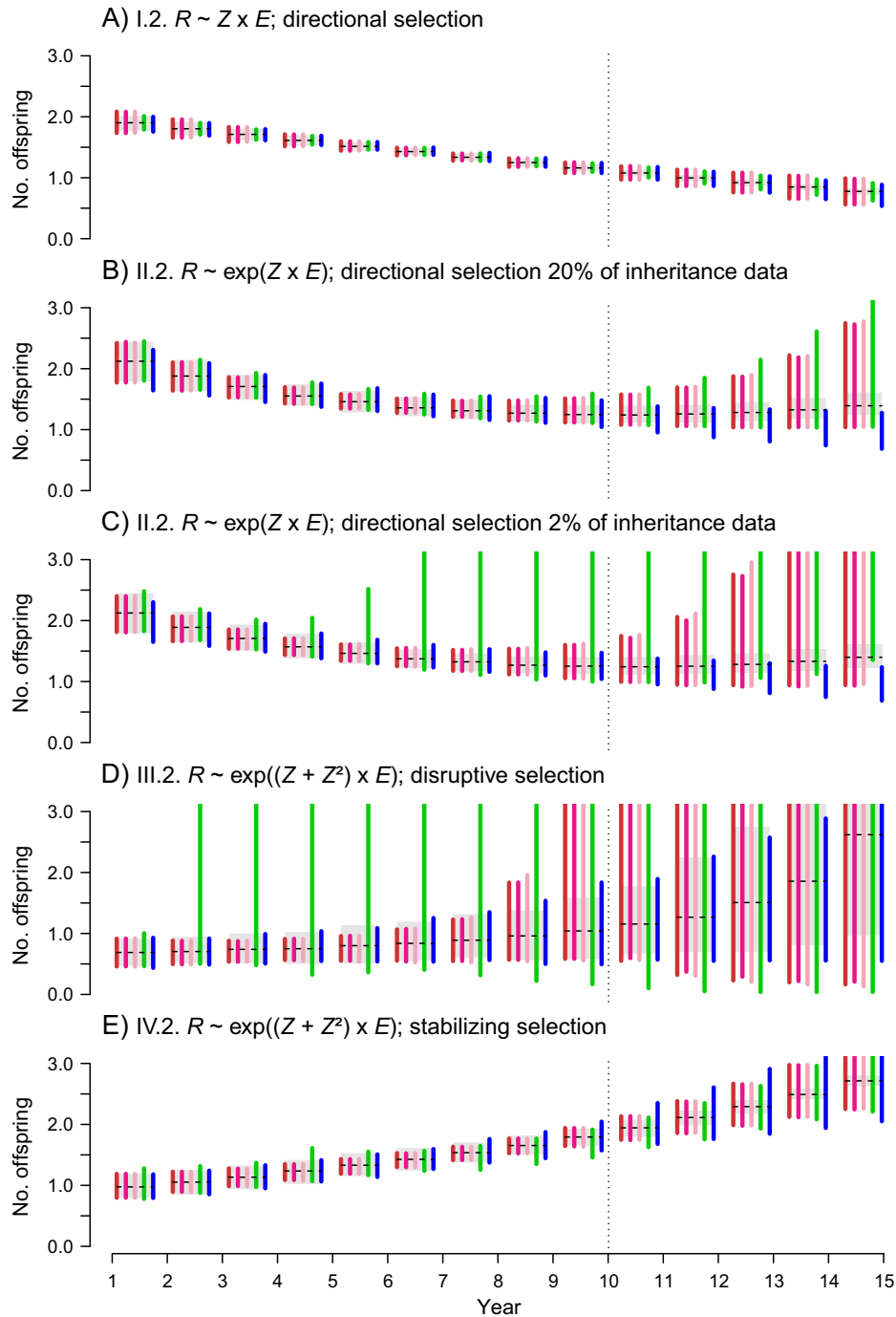
FIG. 5. The 95% confidence intervals of posterior means of estimates of reproductive rates during years 1 to 15 under scenarios I–IV.2 using the five different models: IPM C3 (dark red), IPM C2 (red), IPM C1 (pink), IPM Ind (green), and IPM Pop (blue). Until year 10 (vertical dotted lines), reproductive rates were estimated from data collected under each simulation. After year 10, data were excluded and demographic rates were forecast. Averages and 95% intervals of the true demographic rates estimated over 500 sampled populations are shown by horizontal dashed black lines and gray shades, respectively. For scenario II.2, the results are shown when 20% (B) or 2% (C) of the inheritance data have been collected. In A, D, and E, 20% of the inheritance data have been collected.
